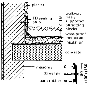
12 Wall connection with FD sealing strip (walkway)
